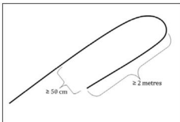
Diagram of the ends of the fence designed to curve inward in order to direct animals away from the area of exclusion (MNRF, 2013)
