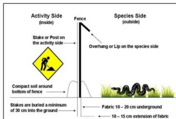
A side view of a basic exclusion fence including an overhang or flexible lip to deter animals from climbing or jumping over the fence. Placement of the stake on the Activity Side or on the inside of excluded area. (MNRF, 2013)
